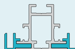
PROFILE CROSS-SECTION WITH RIGID GRAPHIC INSERT ON TWO SIDES
